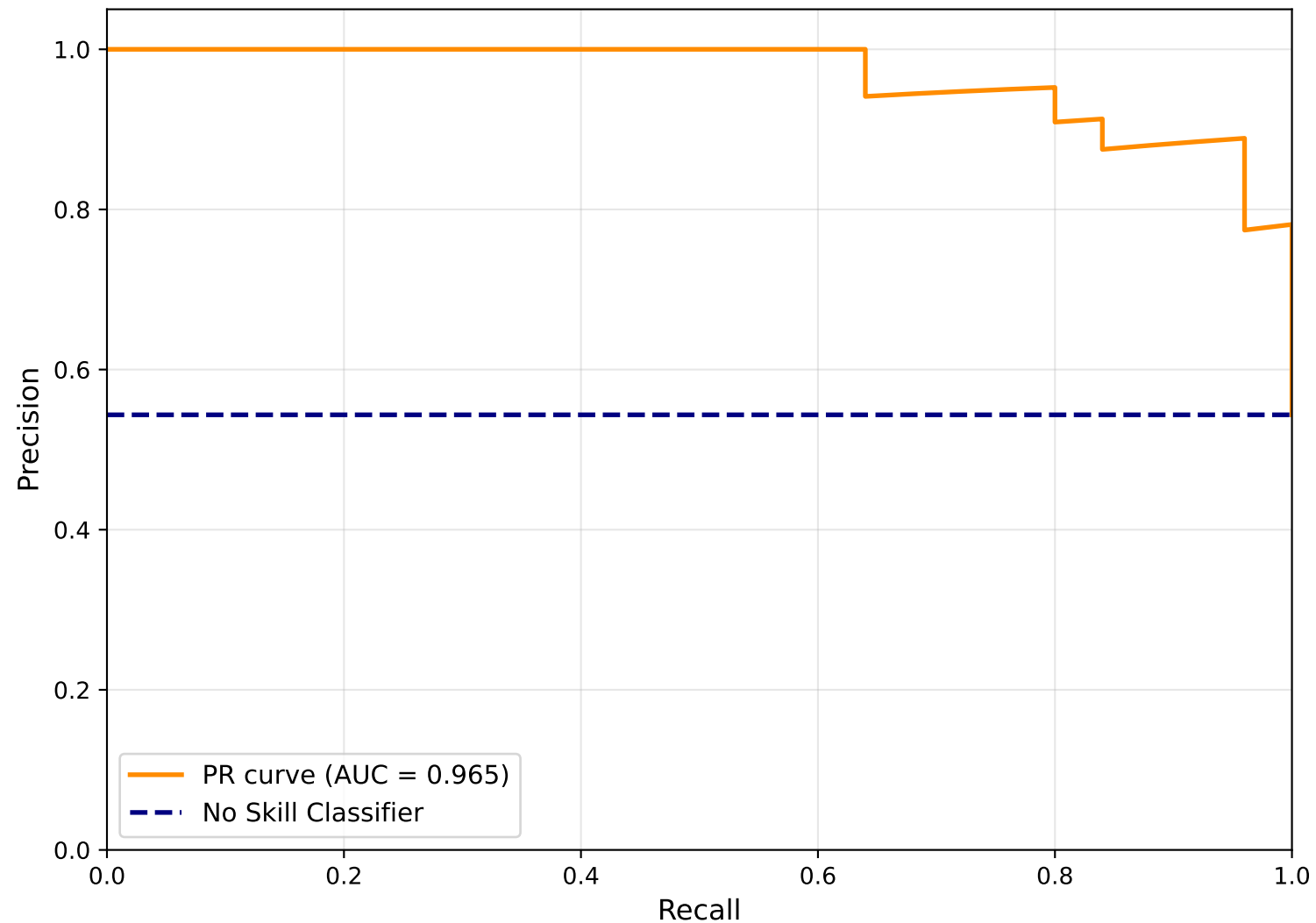
Precision-Recall Curve for Tuned Extra Trees
